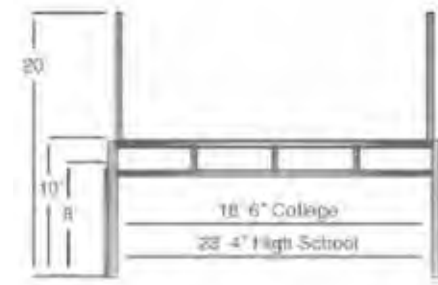
Single Post Pitch Fork Football Goal
