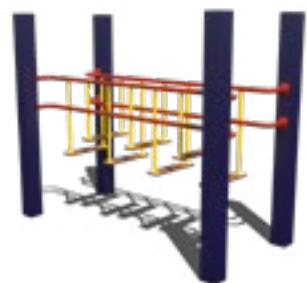
Challenge Bridge TCW06688XX Decks: Equal Height (12"-30") Length: 8' Posts and deck are not included
